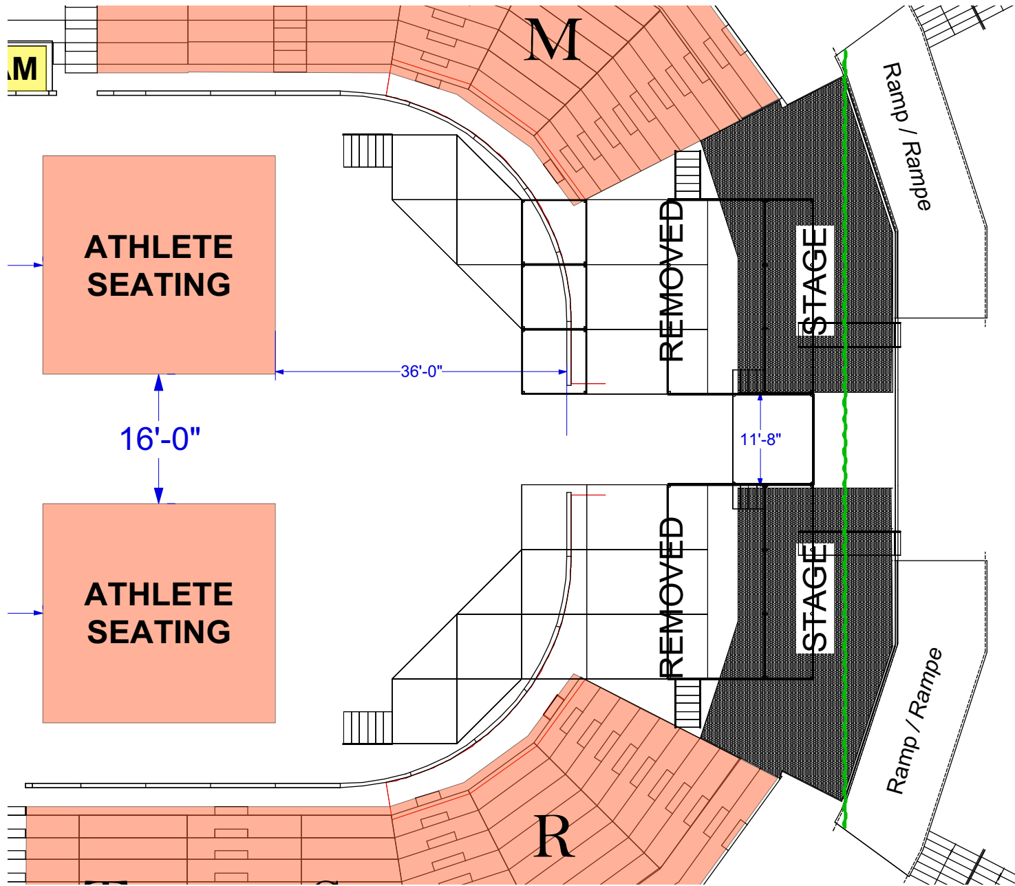
Floor Performance Space Measurements
